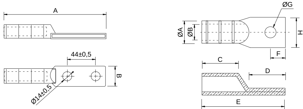
Figura 50 - Conector terminal
